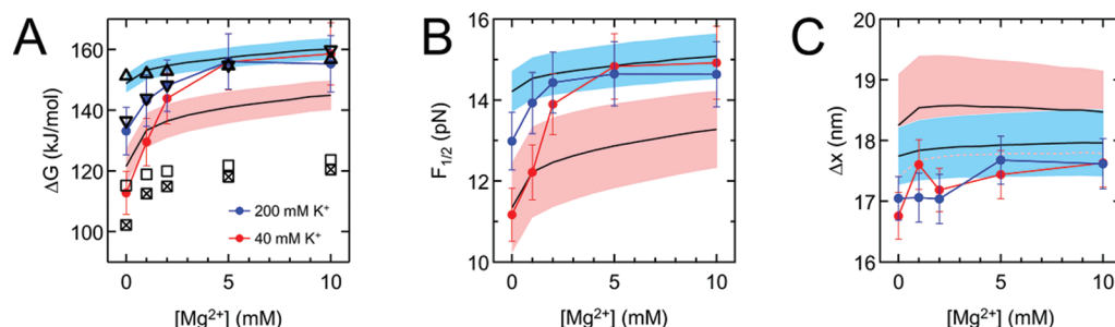
Figure 4. Divalent titrations. \Delta G and \Delta G_{\text{el}} (A), F_{1/2} (B), and \Delta x (C) were measured (circles) and calculated for titrations of \text{Mg}^{2+} against \text{K}^{+} backgrounds. Experimental error bars are as reported in Figure 3. Data points are connected to guide the eye. PB energies (downward and upward-pointing triangles for 40 and 200 mM \text{K}^{+} , respectively) were fitted by \chi^2 minimization to the experimental energies at 5 and 10 mM \text{Mg}^{2+} in each titration. Predictions from the HEL model and mfold are depicted by black traces (uncertainty envelopes for 40 and 200 mM \text{K}^{+} in pink and blue) and squares (crossed and open for 40 and 200 mM \text{K}^{+} , respectively). Values of \Delta x (C) predicted by the HEL model overlapped substantially for the 40 and 200 mM \text{K}^{+} series; a pink dotted line denotes the bottom of the 40 mM uncertainty envelope.
